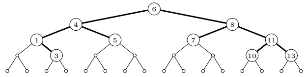
Figure 1: The embedding of a search tree with height 4 and size 10 in a complete tree with height 5
