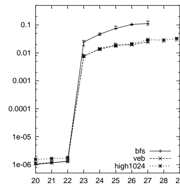
Figure 8: Beyond main memory
