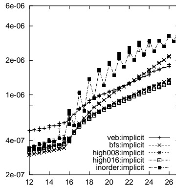
Figure 4: Searches for implicit layouts
