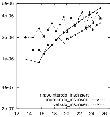
Figure 6: Insert time per element
